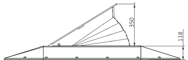
Above the ground installation
